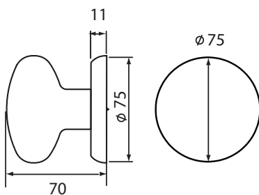
Centre Knob
