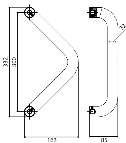
V Handle
