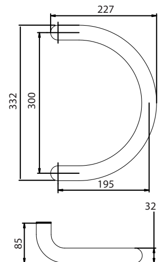
D Handle
